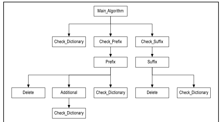
Fig 2. The Hierarchy Chart of The Sub Modules
